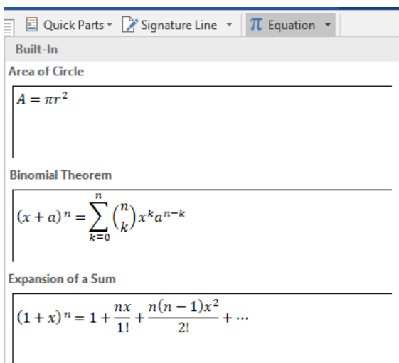
Fig. 2. Adding equations
